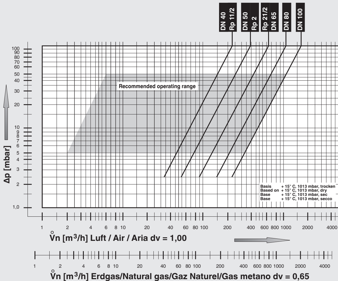
Flow diagram in regulated state
